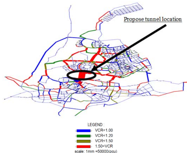
Fig. 17 Route assignment for long term (Option-3)
