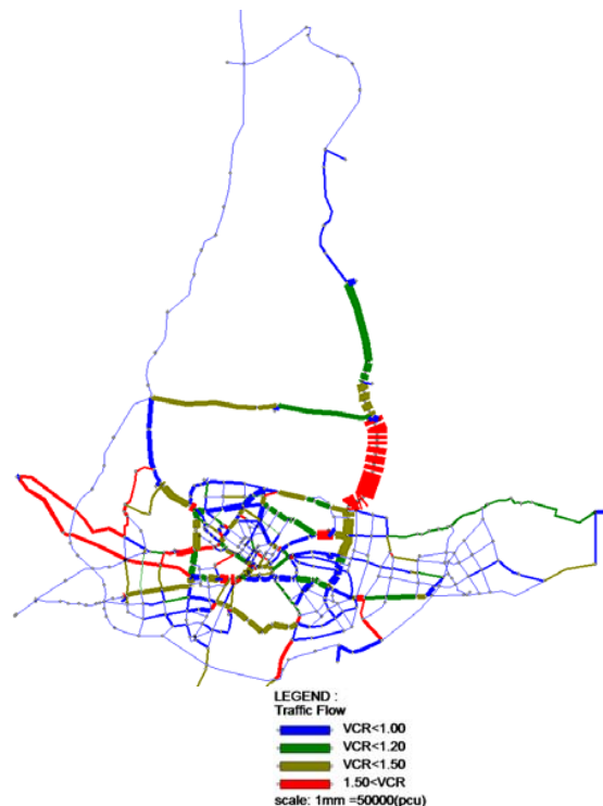
Fig. 5 Route assignment for short term
