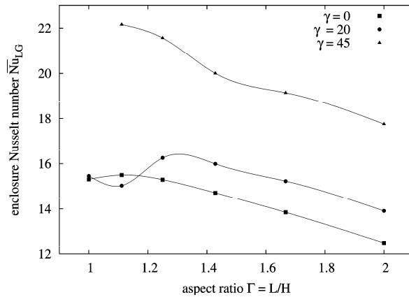
Fig. 10 Enclosure Nusselt number in dependence of the aspect ratio \Gamma and the inclination angle \gamma for an empty enclosure (without heat source). Re = 3800
