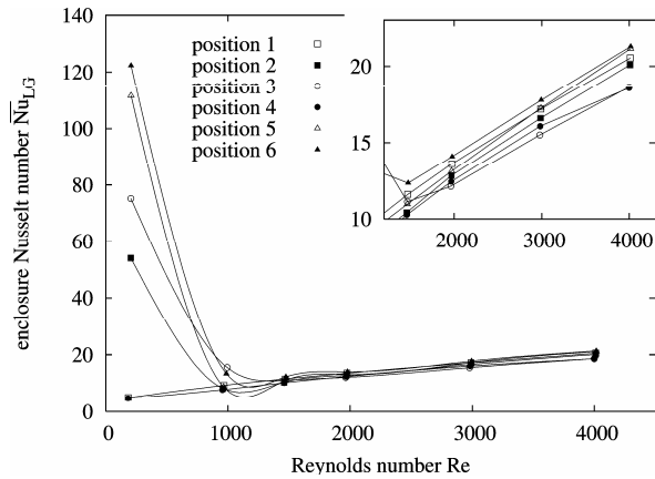
Fig. 6 Enclosure Nusselt number in dependence of the Reynolds number for different positions of the heat source. \Gamma = 1.25 , \gamma = 20^\circ , Gr = 9.5 \cdot 10^6
