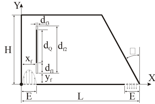
Fig. 2 Measures of the headlight geometry
