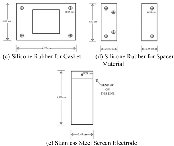
Fig. 2 Required Parts for Single Slice O 2 /H 2 PEMFC
