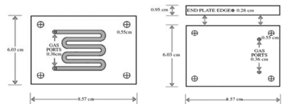
(a) Graphite Serpentine Flow Plate (b) Fiberglass End Plate
