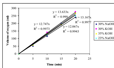
Fig. 4 Volumetric Flow Rate of Oxygen Gas Evolved from the Electrolyzer
