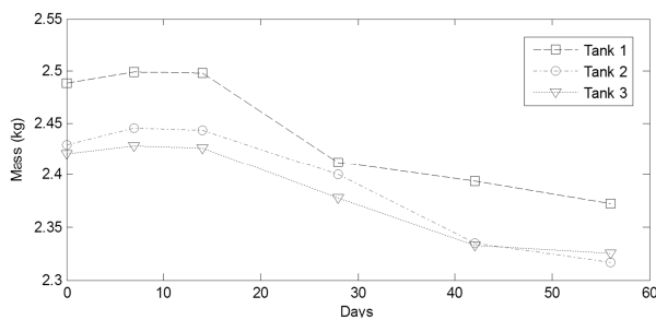
Fig. 3 Average mass of the cubes extracted at different days compared over three temperature regimes of sulphuric acid solution
