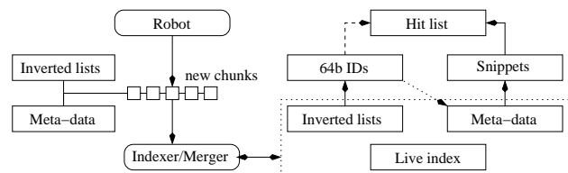
Fig. 1 EGOTHOR architecture
