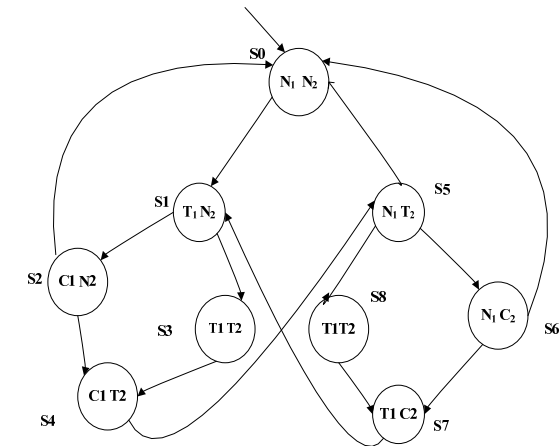
Fig. 4 (a) Model for mutual exclusion
