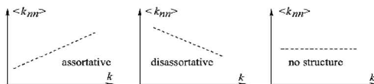
Fig. 1 Assortative / Disassortative Relationship
