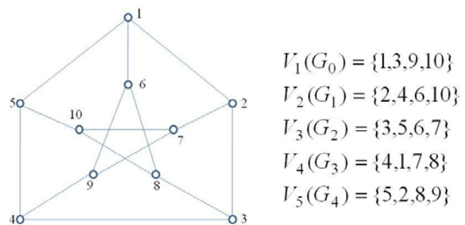
Fig. 2. Thus e(\text{PetersenGraph}) \leq 5 and as choice of every independent set is optimal e(\text{Petersen Graph})=5
