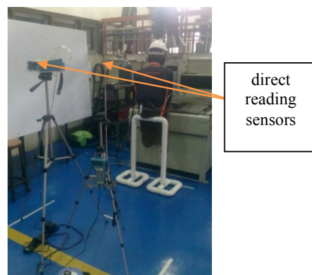
Fig. 3 Direct reading instruments set-up
