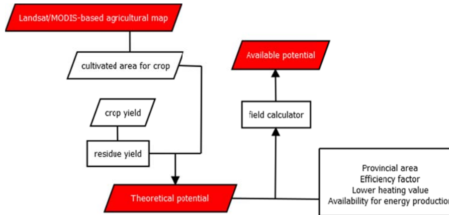
Fig. 3 GIS-based biomass resource assessment workflow
