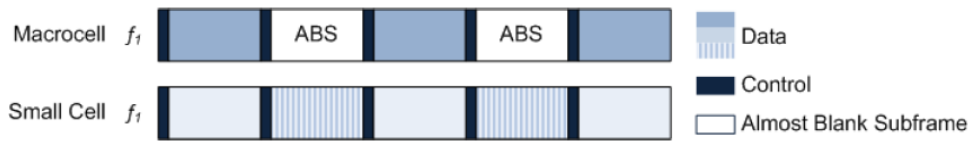
Fig. 8 Time-domain technique based on ABS concept [9]
