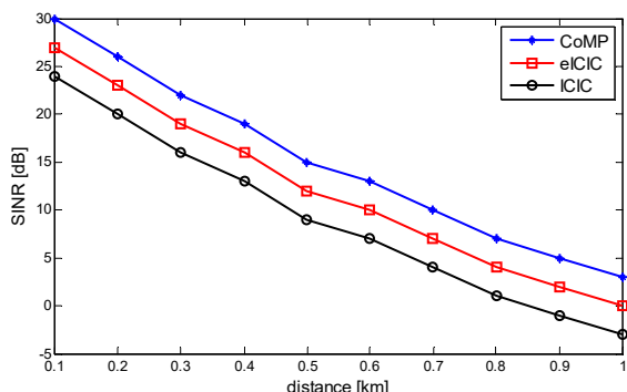
Fig. 10 SINR variation according to the distance for different coordination approaches
