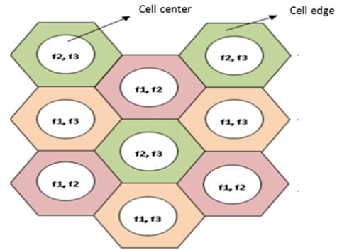
Fig. 7 Fractional Frequency Reuse
