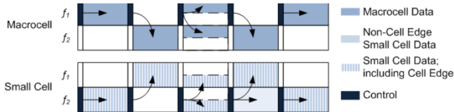
Fig. 9 Frequency-domain technique based on carrier aggregation
