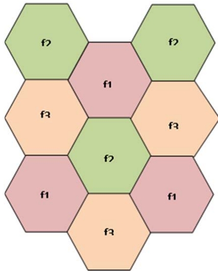
Fig. 5 Hard Frequency Reuse
