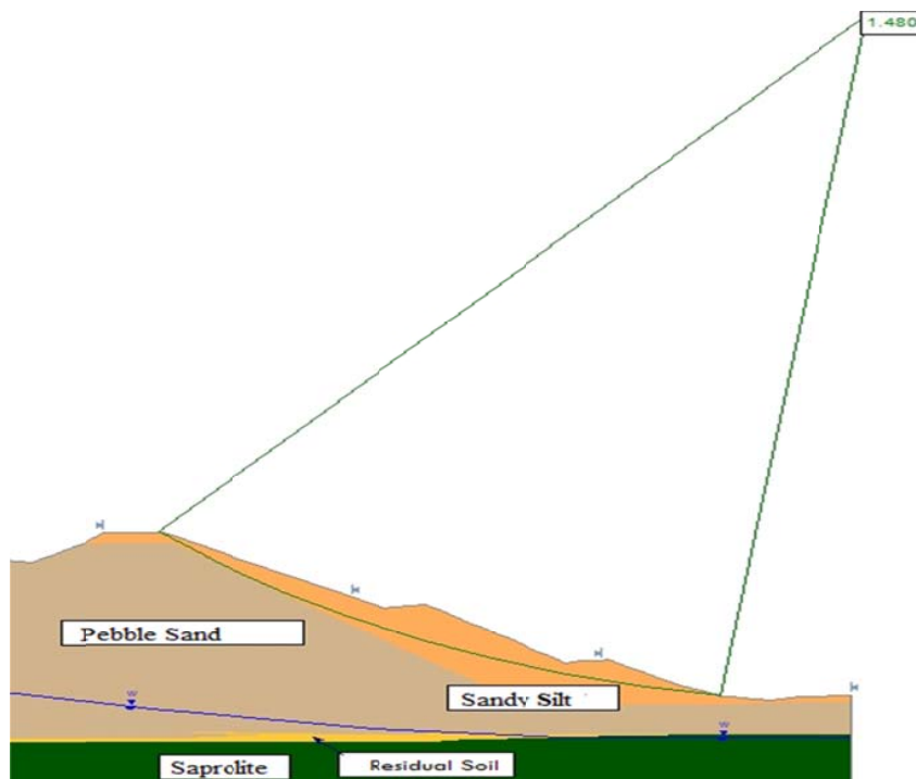
Fig. 5 FS_{\text{medium}} = 1.48 (Deterministic)
