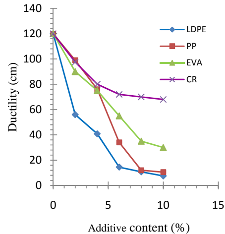
Fig. 7 Effect of polymer additives on ductility
