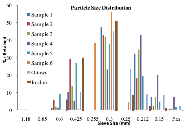
Fig. 4 Particle Size distribution Comparative Graph
