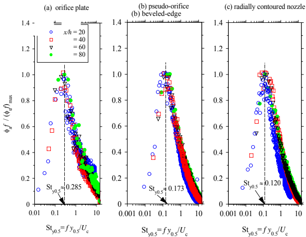
Fig. 9 Far-field evolutions of centreline velocity spectra, \Phi_f / (\Phi_f)_{\max} . (a) orifice plate, (b) pseudo-orifice, (c) radially contoured nozzle
