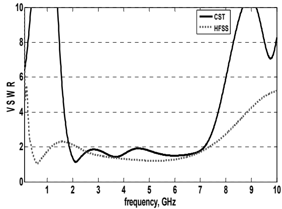
Fig. 6 VSWR of the proposed antenna with CST & HFSS
