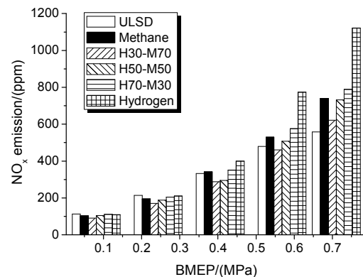
Fig. 7 Effect of hydrogen-methane mixture on \text{NO}_x emission
