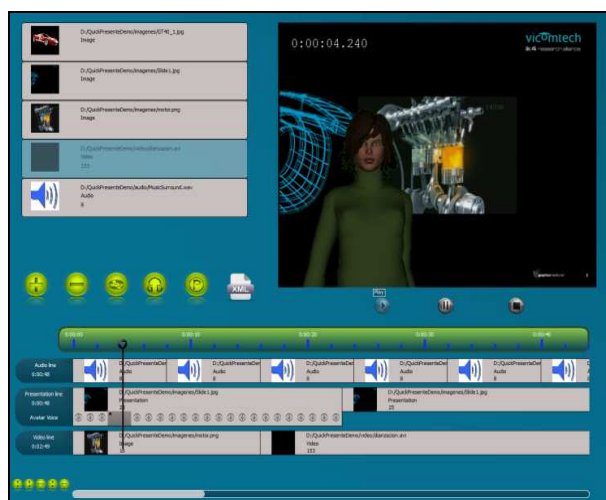
Fig. 1 Video Editor
