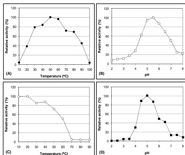
Fig. 5. Effect of temperature and pH on recombinant \beta -glucosidase. A – relative activity of \beta -glucosidase at different temperatures; B – relative activity at different pH; C - effect of temperature on stability of the enzyme; D – enzyme stability at different pH. The relative activity of BGL1 was expressed in percentage of the maximum.
