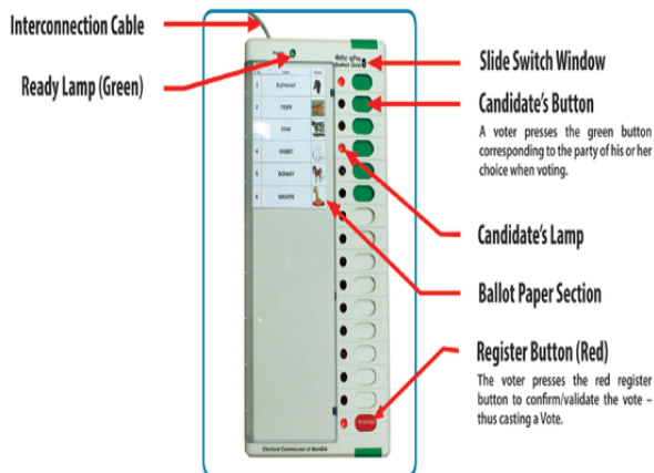
Fig. 3 Ballot Unit [18]
