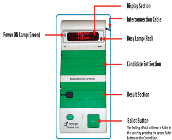
Fig. 2 Control Unit [17]
