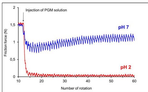
Fig. 5 Friction vs. number of rotations for the sliding contacts between PDMS/PDMS surfaces in buffer solution, followed by injection of mucin solutions (at \sim 12^{\text{th}} rotations)
