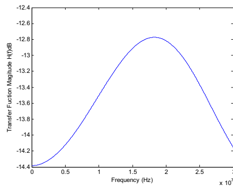
Fig. 15 Transfer Function Plot for Power Line Model with total cable length 4m and bridge tap length 2m with branch impedance 50 \Omega , Z_s = 50\Omega , Z_L = 50\Omega
