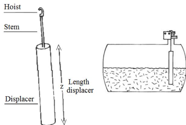
Fig. 1 Displacer typical
