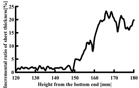
Fig.13 Ratio of Sheet Thickness (Feeding Speed: 50 [mm/min])
