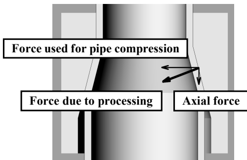
Fig. 2 Processing forces
