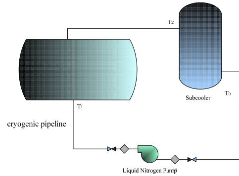
Fig. 5 Flow Chart of a Feed Liquid System
