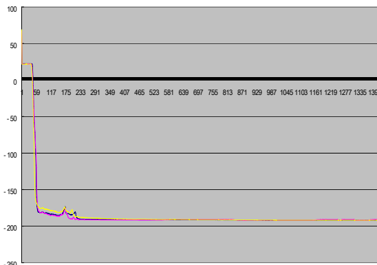
Fig .8 The Pipeline's Cooling Test Curve without Interventions of the Exterior Flow Distribution
