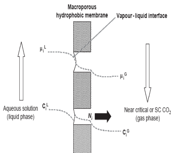
Fig. 1. Principle of mass transfer in porocritical extraction [8].
