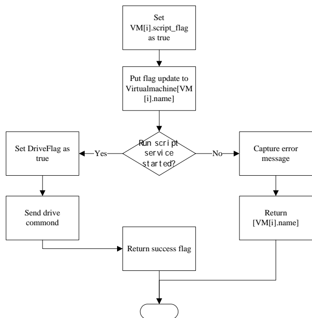
Fig. 2 Control flow in test script execution
