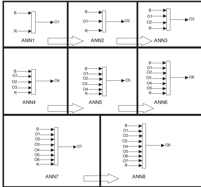
Fig. 4 Proposed ANN System: B: Bias Signal; R: Input Parameters of ANN1; O1: Surface temperature (Co); O2: Current Total Harmonic Distortion (IL1 THD); O3: Current Total Harmonic Distortion (IL2 THD); O4: Current Total Harmonic Distortion (IL3 THD); O5: Voltage Total Harmonic Distortion (VLN1 THD); O6: Voltage Total Harmonic Distortion (VLN2 THD); O7: Voltage Total Harmonic Distortion (VLN3 THD); O8: Interior temperature of induction motor (Co)
