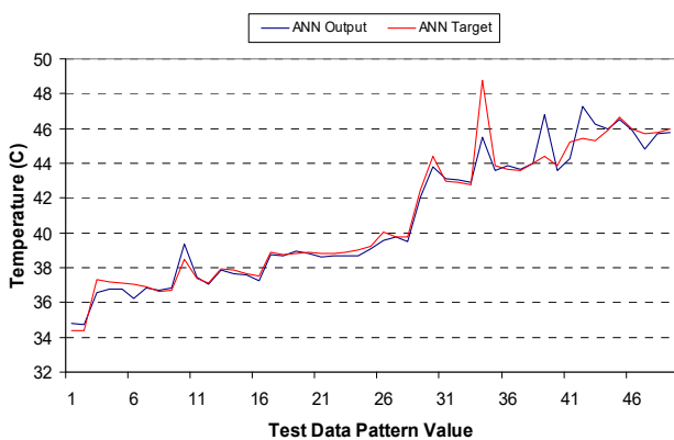
Fig. 8 Comparison of the Cascaded ANN Test Results and Target
