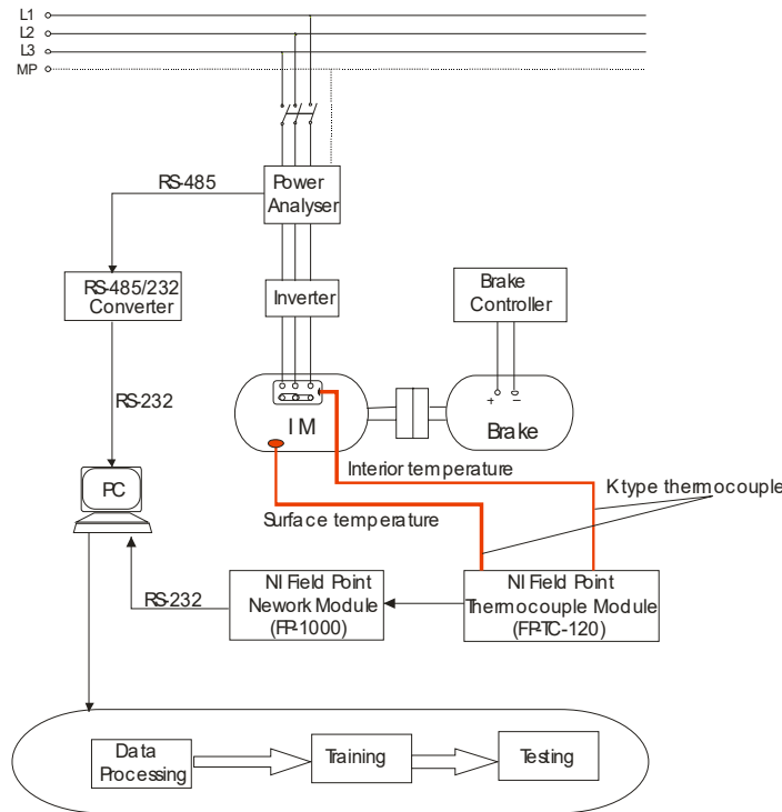
Fig. 2 Experimental Mechanism
