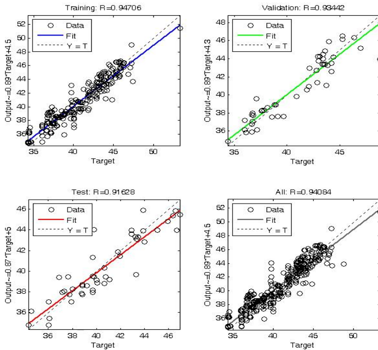
Fig. 6 Regression Graphs of Training, Validation and Testing
