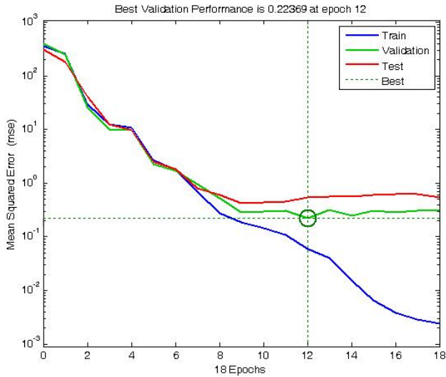
Fig. 9 Performance of the Cascaded ANN System
