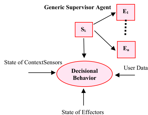
Fig.1. Schema of a Generic Supervisor Agent
