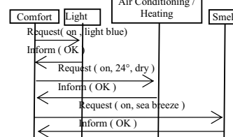
Fig.4. Exchange of ACL messages
