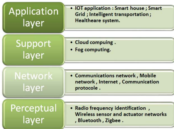
Fig. 2 IoT Architecture
