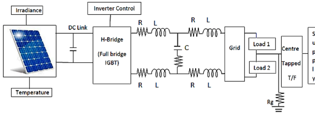
Fig. 8 Schematic model of Transformer less PV system with LCL configuration connected to Utility Grid
