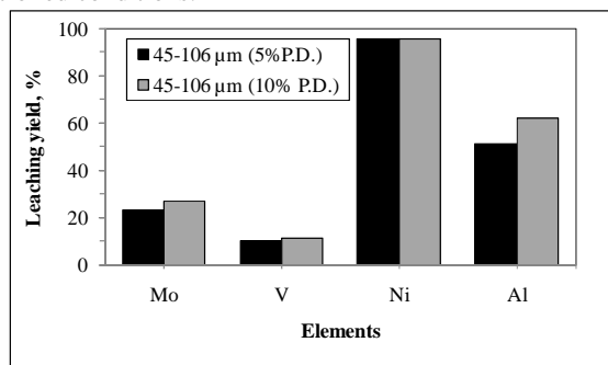
Fig. 7 Comparative leaching yield between 5% and 10% P.D. at a size fraction of 45-106 \mu\text{m}
