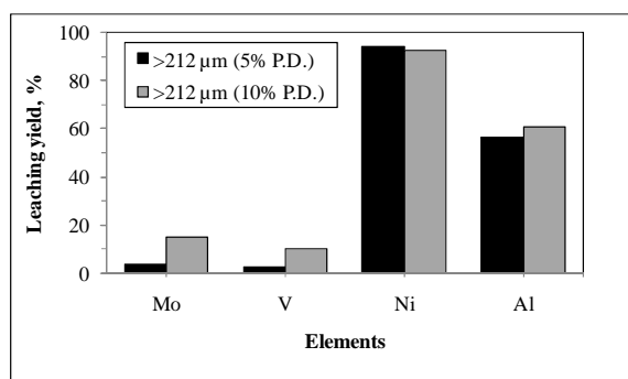
Fig. 9 Comparative leaching yield between 5% and 10% P.D. at a size fraction of \geq 212 µm
