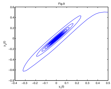
Fig.7-9. Behavior and phase portrait of system (53) with \tau = 3.6, \sigma = 0.5 < \sigma_0 \approx 0.6488 . The equilibrium E_0(0, 0) is asymptotically stable. The initial value is (0.2, 0.2) .
