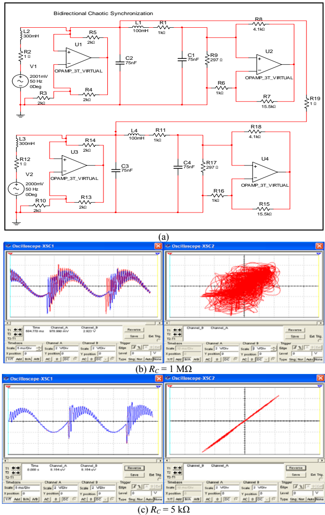
Fig. 6 MultiSIM ® Circuit and simulations: (a) Synchronization of chaotic non-autonomous attractor Circuit; (b) Drive and response system chaotic signals before synchronization; and the phase portrait of unsynchronized case; (c) Drive and response system chaotic signals after synchronization; and X-Xr Synchronization
