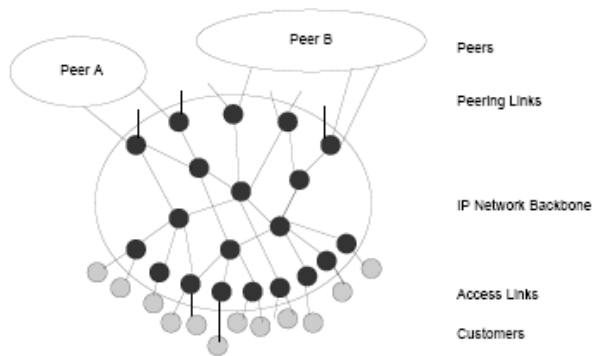
Fig. 1. IP network components and terminologies.
