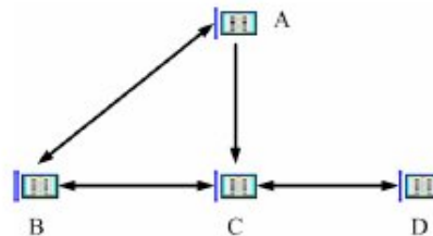
Fig. 2. 4-Node Topology
