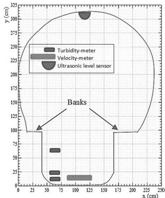
Fig. 1 Sewer Section Details and Measurement Equipment Position
