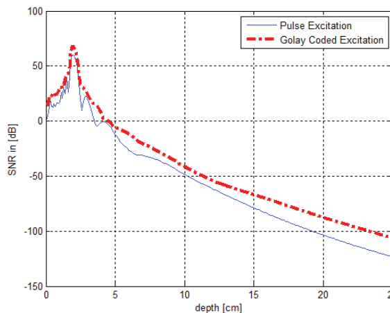
Fig. 8 Simulation results on the SNR for sinusoidal burst and a Golay coded signal under presence of attenuation and absence of randomly positioned scatterers. Matched filtering is applied
