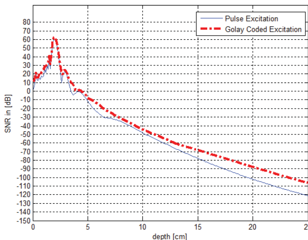
Fig. 7 Simulation results on the SNR for sinusoidal burst and a Golay coded signal under presence of attenuation and absence of randomly positioned scatterers in the simulated medium
