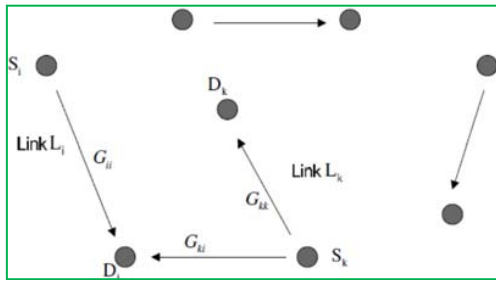
Fig. 9 Scheduling Process
