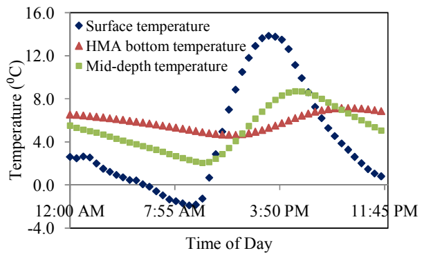
Fig. 11 Variations of temperature with time
