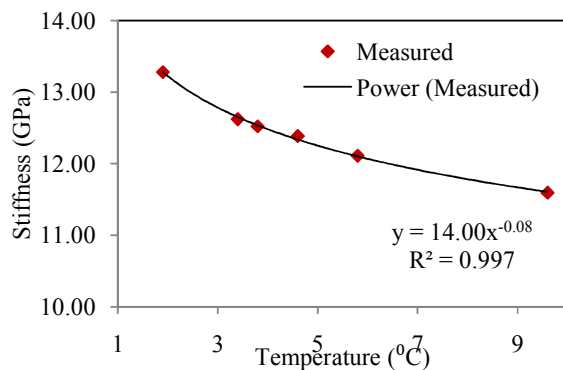
Fig. 13 Stiffness variations with mid-depth HMA temperatures
