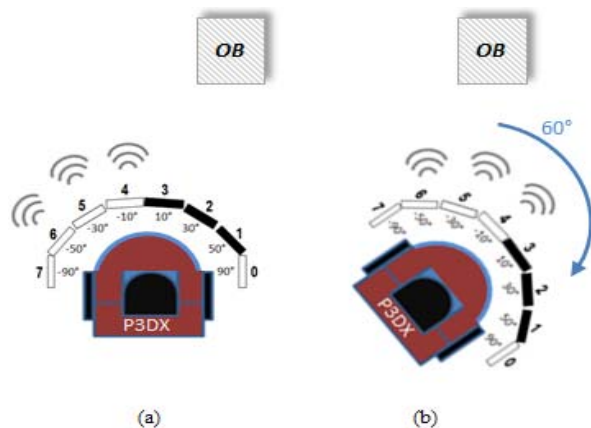
Fig. 8 Sonar sensors (1-3) as disabled (a); they are 'blind' to object OB. The Compensation Policy is used to establish that a 60° clockwise rotation (b), can allow the P3-DX robot to detect object OB
