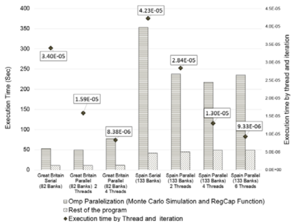
Fig. 14 Thread time characterization for medium inputs
