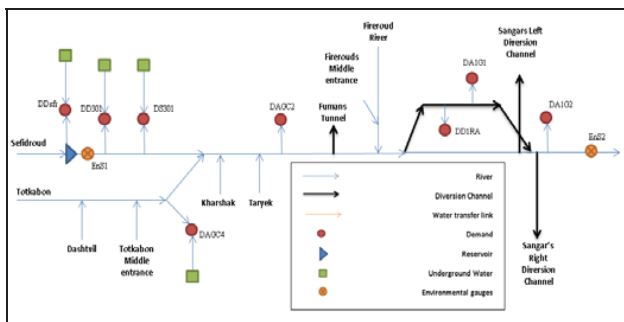
Fig. 2 Node-link schematic view of Sefidroud River system
