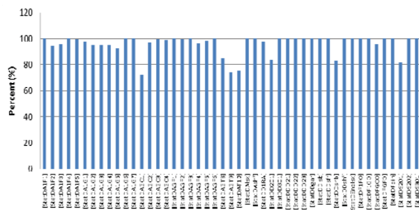
Fig. 5 Demand satisfaction for major demand sites in Gilan's water resource system
