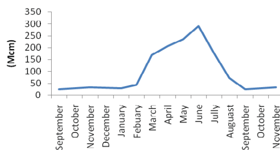
Fig. 6 Sefidroud's reservoir monthly average rule curve
