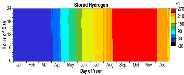
Fig. 7 The yearly hydrogen tank storage level
