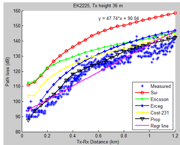
Fig. 8 Comparison of observed path losses in urban environment with proposed two slope, SUI, Ericson, Cost 231-Hata and Ercege models
