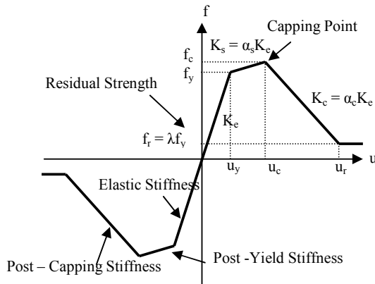
Fig. 1 Backbone curve of deteriorating hysteretic model [3]
