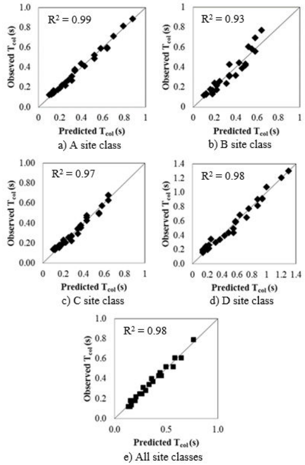
Fig. 4 Observed and predicted T_{col} for different site classes and moderate degradation ( \gamma = 100 )
