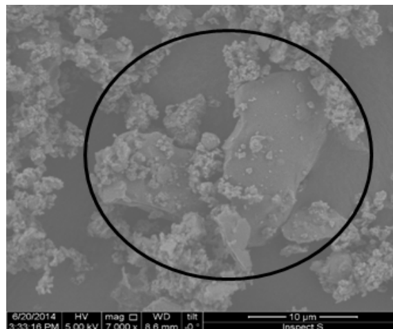
Fig. 4 SEM Image of CWM
