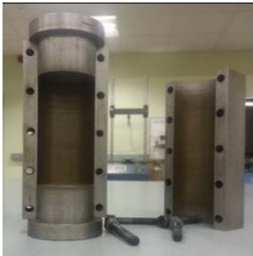
Fig. 6 Constant Volume Mould Used to Prepare the Soil Specimens for UCS Tests
