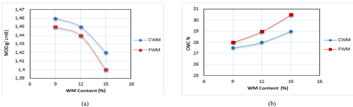
Fig. 10 Effect of Fineness of WM on the Compaction Parameters: (a) MDD, and (b) OMC
