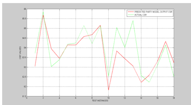
Fig. 6 NN output For Coal Characterization Prediction Model
