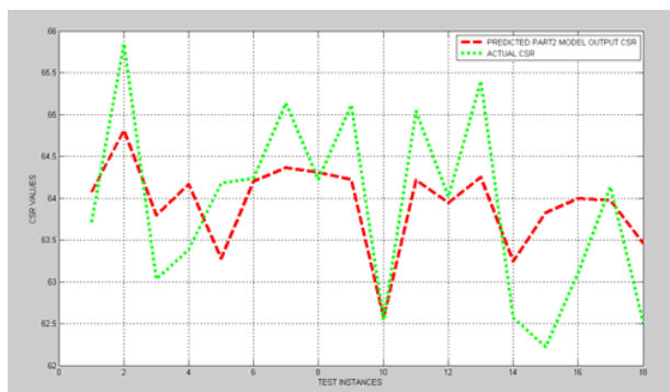
Fig. 7 NN Output For Coke Process Prediction Model
