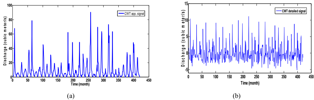
Fig. 1 Signal decomposing into the approximation and the detail signal using CWT transforms (a) Band-e-Bahman CWT based approximation signal (b) Band-e-Bahman CWT based detail signal
