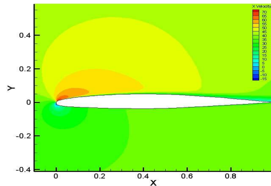
Fig. 2 (b) Velocity distribution on clean GLC305 at AoA = 8° M = 0.12, Re = 3x10 6
