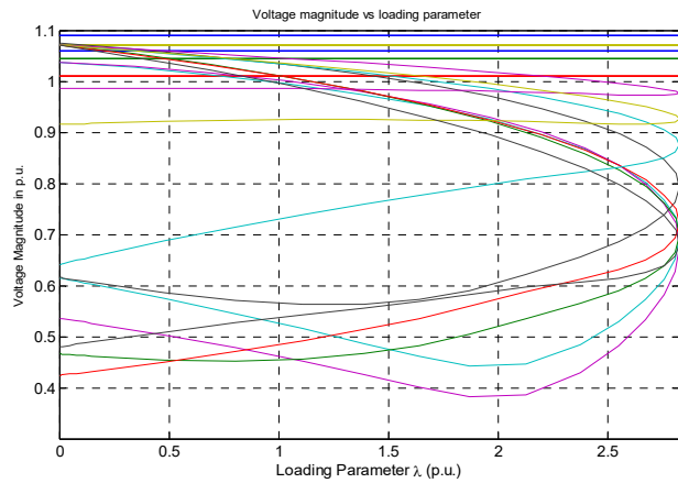
Fig. 9 Loadability margin without STATCOM
